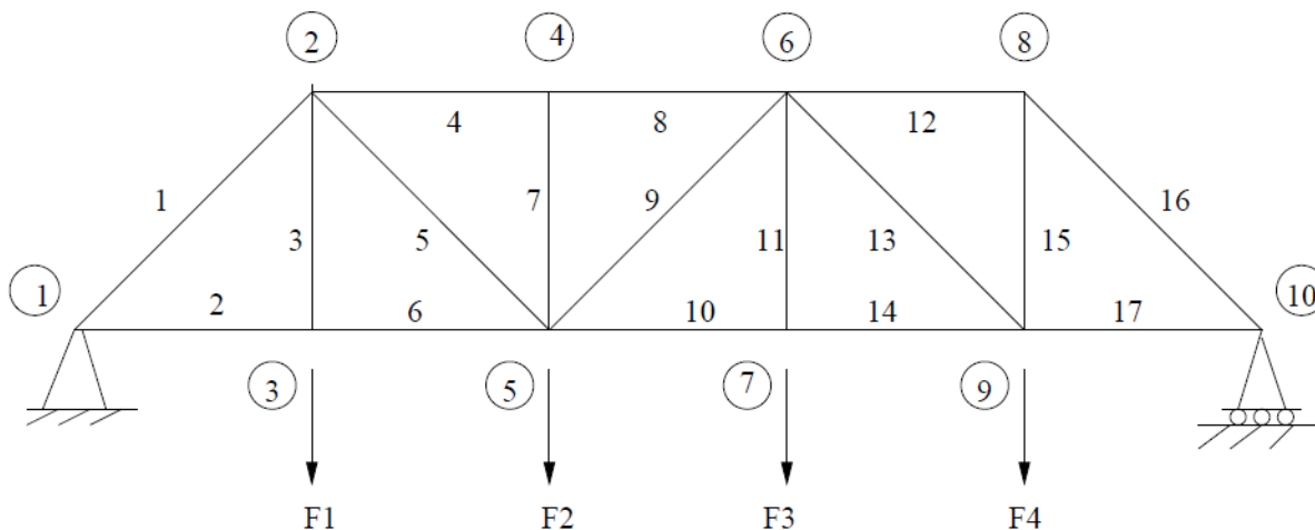
Figure 1: Schematic of the truss structure.
